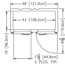
Plan - UR48HT
