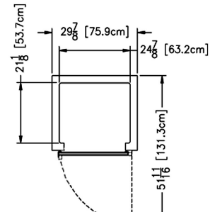
Plan - R/AHT126WUT
