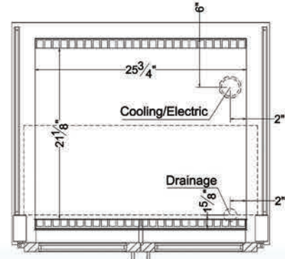
LARGEST DIMENSION REPRESENTS OUTSIDE FLANGE
