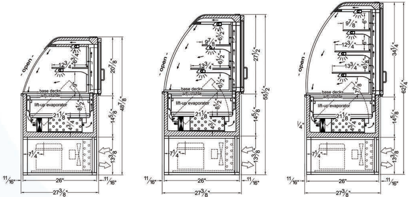
UNITS SHOWN WITH "REAR AIR BREATHING" OPTION
