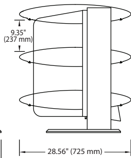
SIDE VIEW Horizontal
