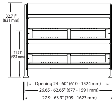
FRONT VIEW Slant
