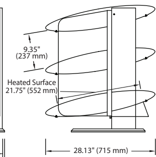
SIDE VIEW Slant
