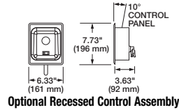
Optional Recessed Control Assembly
