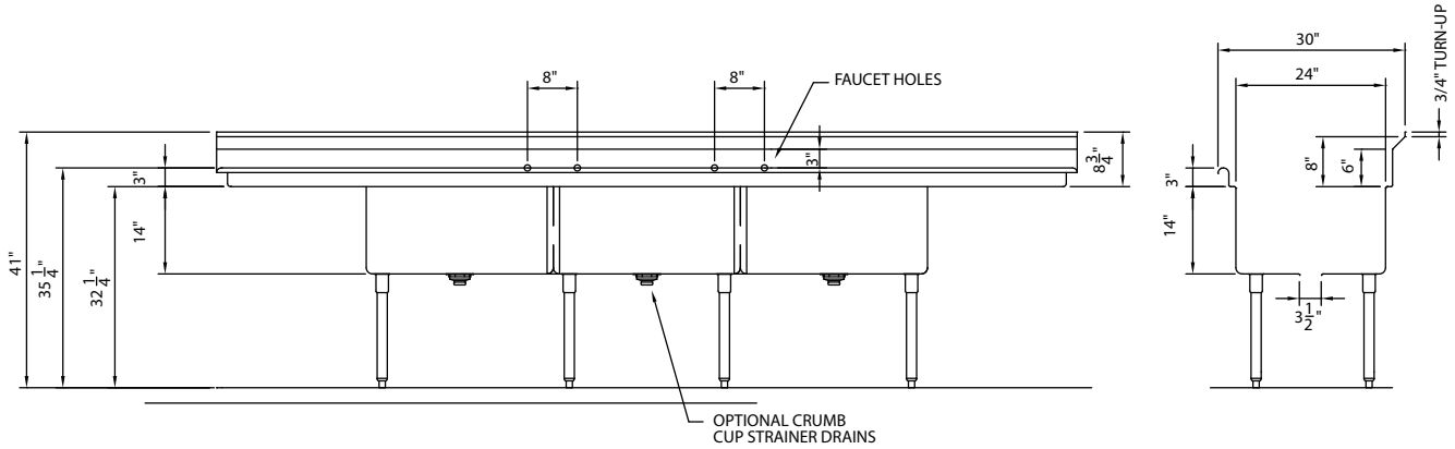
FRONT VIEW
