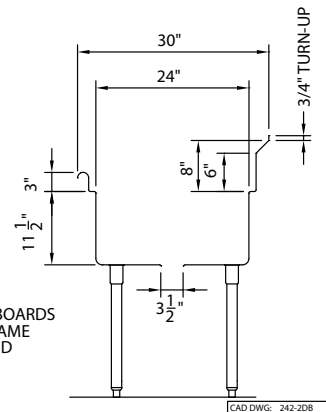
SECTION VIEW
