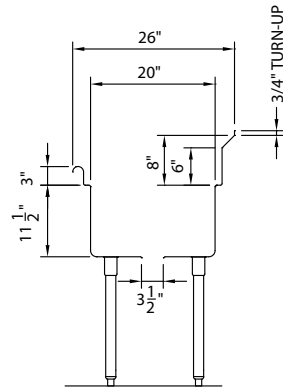
SECTION VIEW
