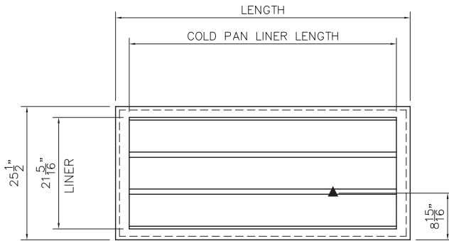
ADI-4M-TC UNIT SHOWN
