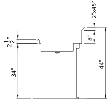
SECTION A
