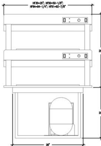
MODEL HF50-2 Capacity: Six (6) 13" x 26" sheet pans. (Self-contained refrigeration system required for frost applications)
