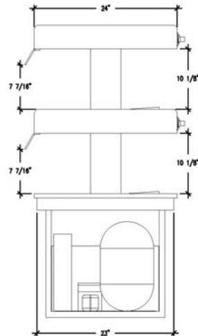
MODEL HF64-2 Capacity: Four (4) 18" x 26" sheet pans. (Self-contained refrigeration system required for frost applications)
